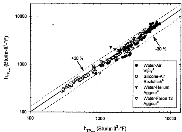
Fig. 1 Comparison of the new correlation [Eq. (13)] with all of the two-phase heat transfer experimental data (255 data points) in Table 1.
